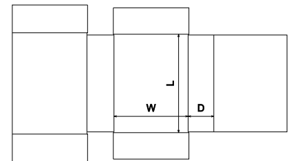
FEFCO Corrugated\0400 - Folder Type Boxes\ FEFCO 0497 - 5 Panel Folder - Non-Glued
