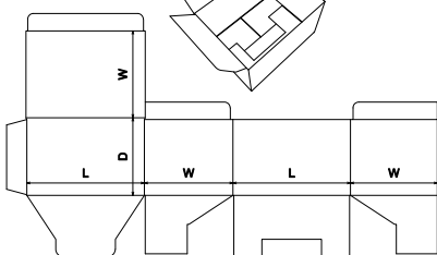
FEFCO Corrugated\0200 - Slotted Type Boxes\ FEFCO 0215 - Tuck to Front Top, Envelope Base
