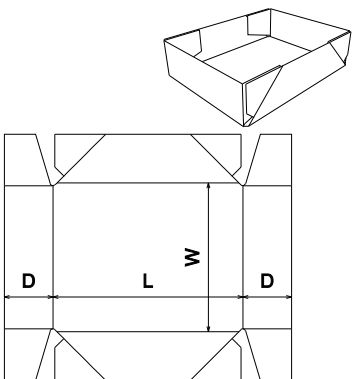
FEFCO Corrugated\0400 - Folder Type Boxes\ FEFCO 0451 - Infold Tray
