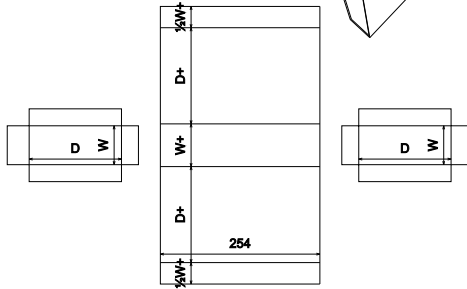
FEFCO Corrugated\0600 - Rigid Type Boxes - Bliss Boxes\FEFCO 0620 - Wrap with Internal Side Caps
