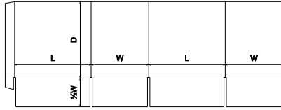
FEFCO Corrugated\0200 - Slotted Type Boxes\ FEFCO 0200 EF - Half Slotted Container Extended Flaps - HSC EF
