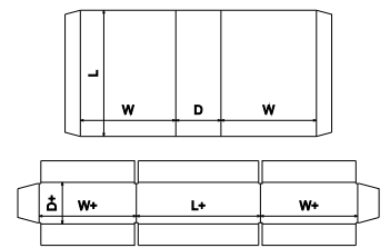
FEFCO Corrugated\0500 - Slide Type Boxes\ FEFCO 0512 - Interlocking Sleeves Side Glued
