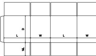
FEFCO Corrugated\0200 - Slotted Type Boxes\ FEFCO 0205 - End Flaps Meet Slotted Container - CSO EFM
