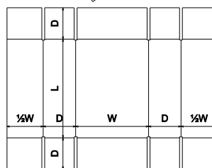
FEFCO Corrugated\0400 - Folder Type Boxes\ FEFCO 0411 - Five Panel Folder, Centre Seam - FPF
