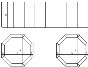
FEFCO Corrugated\0300 - Telescope Type Box\ FEFCO 0350 - Octagonal Bulk Box - Glued Ends
