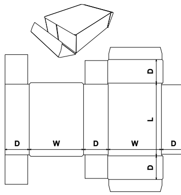
FEFCO Corrugated\0400 - Folder Type Boxes\ FEFCO 0447 - Unglued End Tuck
