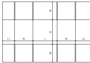
FEFCO Corrugated\0200 - Slotted Type Boxes\ FEFCO 0230 - Full Overlapping Container, Centre Seam on Sides
