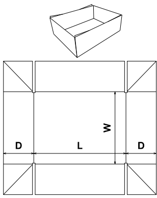
FEFCO Corrugated\0400 - Folder Type Boxes\ FEFCO 0448 - Outfold Tray, Side Slots
