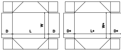
FEFCO Corrugated\0300 - Telescope Type Box\ FEFCO 0303 - Outfold Tray and Lid
