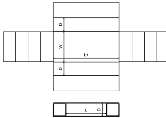
FEFCO Corrugated\0400 - Folder Type Boxes\ FEFCO 0403 - One Piece Folder Buffer Ends - Air Cell
