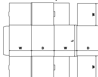
FEFCO Corrugated\0400 - Folder Type Boxes\ FEFCO 0470 - Economy Tray RE Tuck Top
