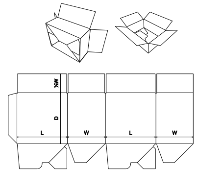
FEFCO Corrugated\0700 - Ready Glued - Self-Erecting Boxes\FEFCO 0711 - Crash Lock Auto Bottom, Regular Slotted Top - CLB/RSC
