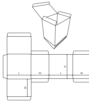
FEFCO Corrugated\0200 - Slotted Type Boxes\ FEFCO 0210 - Aeroplane Tuck, Tuck to Front Container
