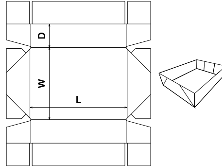
FEFCO Corrugated\0700 - Ready Glued - Self-Erecting Boxes\FEFCO 0718 - 4 Point Glued Tray
