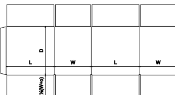
FEFCO Corrugated\0200 - Slotted Type Boxes\ FEFCO 0202 - Overlap Slotted Container - POL
