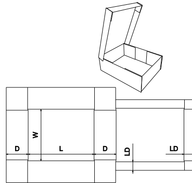
FEFCO Corrugated\0400 - Folder Type Boxes\ FEFCO 0441 - Slitted Tray and Lid
