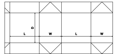
FEFCO Corrugated\0200 - Slotted Type Boxes\ FEFCO 0226 - Bellows Style Container
