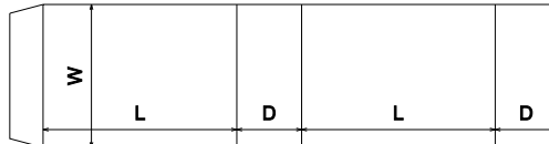
FEFCO Corrugated\0500 - Slide Type Boxes\ FEFCO 0502 - Sleeve - Top, Base and Ends
