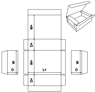
FEFCO Corrugated\0600 - Rigid Type Boxes - Bliss Boxes\FEFCO 0602 - Bliss Box Tuck
