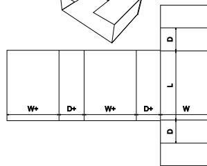
FEFCO Corrugated\0400 - Folder Type Boxes\ FEFCO 0400 - One Piece Folder, Wrap Around - OPF
