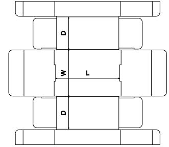
FEFCO Corrugated\0400 - Folder Type Boxes\ FEFCO 0431 - Reinforced Flanged Tray
