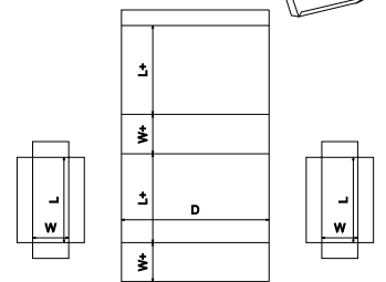
FEFCO Corrugated\0600 - Rigid Type Boxes - Bliss Boxes\FEFCO 0616 - Wrap with Internal Buffer End Caps
