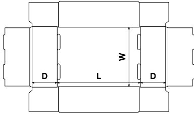
FEFCO Corrugated\0400 - Folder Type Boxes\ FEFCO 0422 - Rolled End Tray
