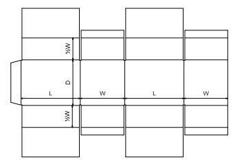
FEFCO Corrugated\0200 - Slotted Type Boxes\ FEFCO 0229 - All Flaps Meet, Centre Partition
