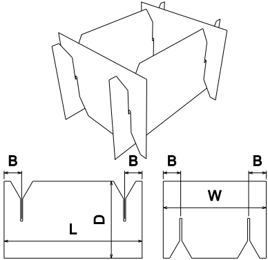
FEFCO Corrugated\0900 - Interior Fitments\ FEFCO 0931 - Interior Compartment with Side Ruffles
