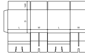
FEFCO Corrugated\0200 - Slotted Type Boxes\ FEFCO 0207 - Slotted Container with Dividers - RSC
