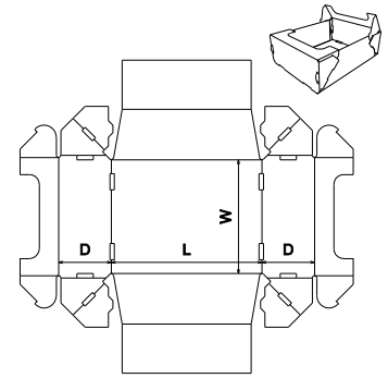
FEFCO Corrugated\0700 - Ready Glued - Self-Erecting Boxes\FEFCO 0774 - Flange Top Tray, Double Sides
