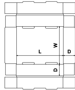
FEFCO Corrugated\0400 - Folder Type Boxes\ FEFCO 0424 - Rolled Side Tray, Reinforced Ends
