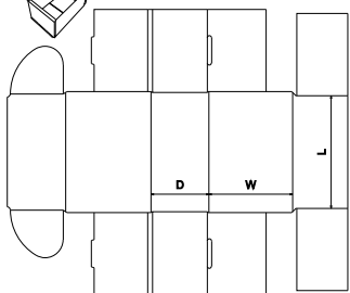
FEFCO Corrugated\0400 - Folder Type Boxes\ FEFCO 0471 - Economy Tray RE Tuck Top CL
