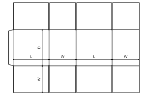
FEFCO Corrugated\0200 - Slotted Type Boxes\ FEFCO 0203 - Full Overlap Slotted Container - FOL
