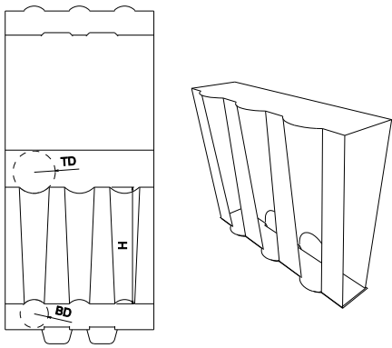
FEFCO Corrugated\0700 - Ready Glued - Self-Erecting Boxes\FEFCO 0752 - Glass Pack
