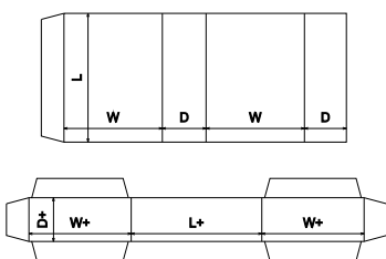
FEFCO Corrugated\0500 - Slide Type Boxes\ FEFCO 0511 - Interlocking Sleeves Inner Tuck with Dust Flaps
