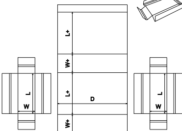
FEFCO Corrugated\0600 - Rigid Type Boxes - Bliss Boxes\FEFCO 0615 - Wrap with Full Cover Buffer End Caps
