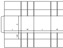
FEFCO Corrugated\0200 - Slotted Type Boxes\ FEFCO 0208 - Slotted Containers with Holders
