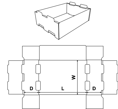
FEFCO Corrugated\0400 - Folder Type Boxes\ FEFCO 0435 - Rolled End Stacking Tray
