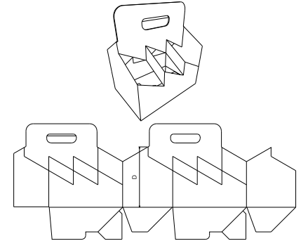
FEFCO Corrugated\0700 - Ready Glued - Self-Erecting Boxes\FEFCO 0717 - Crash Lock Base Auto Bottom, Bottle Carrier - CLB
