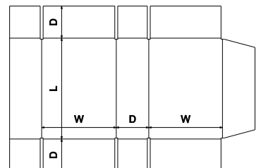
FEFCO Corrugated\0400 - Folder Type Boxes\ FEFCO 0410 - Five Panel Folder - FPF
