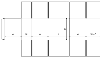
FEFCO Corrugated\0200 - Slotted Type Boxes\ FEFCO 0228 - Full Overlapping Container, Centre Seam, Centre Divider
