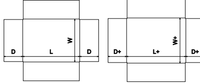
FEFCO Corrugated\0300 - Telescope Type Box\ FEFCO 0302 - Taped Tray and Lid
