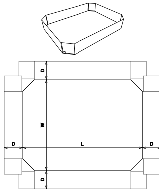
FEFCO Corrugated\0400 - Folder Type Boxes\ FEFCO 0459 - Can Tray
