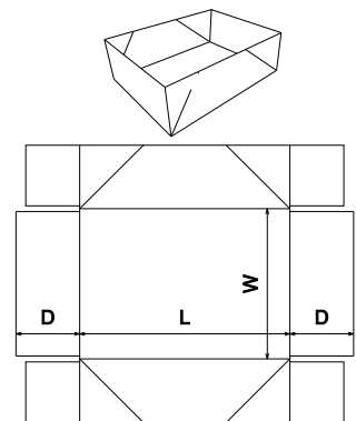
FEFCO Corrugated\0400 - Folder Type Boxes\ FEFCO 0450 - Outfold Tray, End Slots
