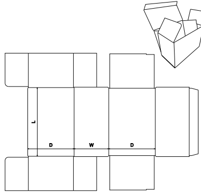
FEFCO Corrugated\0400 - Folder Type Boxes\ FEFCO 0444 - Unglued Tuck To Back
