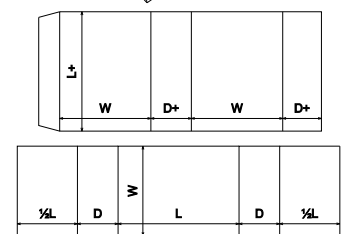
FEFCO Corrugated\0500 - Slide Type Boxes\ FEFCO 0509 - Interlocking Sleeves Inner Centre Join
