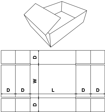
FEFCO Corrugated\0400 - Folder Type Boxes\ FEFCO 0454 - Tray Folded Ends
