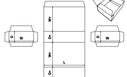
FEFCO Corrugated\0600 - Rigid Type Boxes - Bliss Boxes\FEFCO 0608 - Tuck Wrap with Internal End Caps
