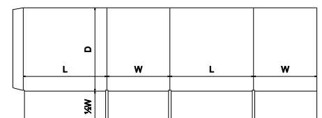
FEFCO Corrugated\0200 - Slotted Type Boxes\ FEFCO 0200 - Half Slotted Container - HSC
