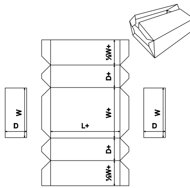
FEFCO Corrugated\0600 - Rigid Type Boxes - Bliss Boxes\FEFCO 0606 - Bliss Box Centre Seam
