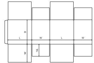
FEFCO Corrugated\0200 - Slotted Type Boxes\ FEFCO 0206 - Overlap Sides, End Flaps Meet - SFF EFM
