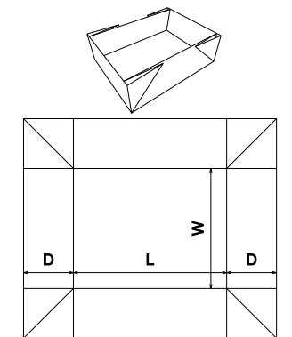
FEFCO Corrugated\0400 - Folder Type Boxes\ FEFCO 0449 - Infold Tray Webbed Corners
