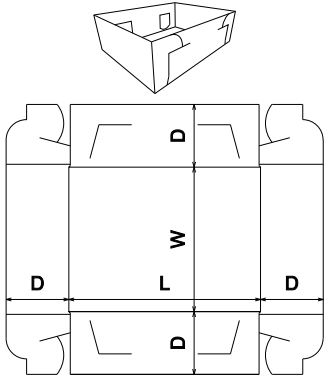
FEFCO Corrugated\0400 - Folder Type Boxes\ FEFCO 0457 - Self Locking Tray
