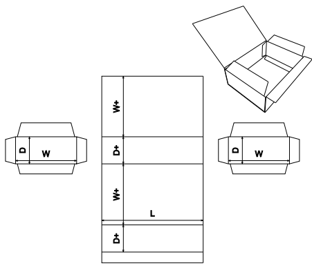
FEFCO Corrugated\0600 - Rigid Type Boxes - Bliss Boxes\FEFCO 0607 - Wrap with Internal End Caps
