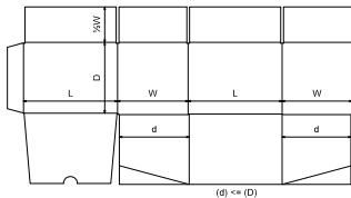
FEFCO Corrugated\0200 - Slotted Type Boxes\ FEFCO 0225 - File Base Slotted Container - RSC
