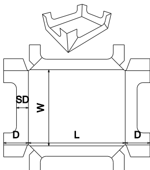
FEFCO Corrugated\0700 - Ready Glued - Self-Erecting Boxes\FEFCO 0770 - Open Sided Tray
