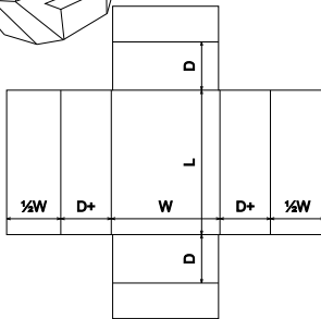
FEFCO Corrugated\0400 - Folder Type Boxes\ FEFCO 0401 - One Piece Folder, Widths Meet - OPF
