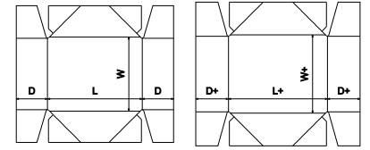
FEFCO Corrugated\0300 - Telescope Type Box\ FEFCO 0304 - Infold Tray and Lid
