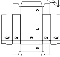
FEFCO Corrugated\0400 - Folder Type Boxes\ FEFCO 0415 - One Piece Taped Folder with Dust Flaps - OPF
