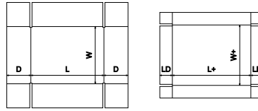
FEFCO Corrugated\0300 - Telescope Type Box\ FEFCO 0306 - Side Slotted Tray with End Slotted Cover
