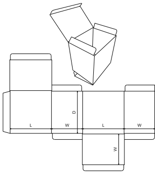
FEFCO Corrugated\0200 - Slotted Type Boxes\ FEFCO 0211 - Reverse Tuck End, Tuck to Front Top, Tuck to Back Base
