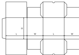
FEFCO Corrugated\0200 - Slotted Type Boxes\ FEFCO 0227 - Slotted Tuck Top and Base
