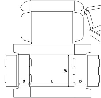
FEFCO Corrugated\0400 - Folder Type Boxes\ FEFCO 0427 - Rolled End Tuck Tray, Dust Flaps and Cherry Locks
