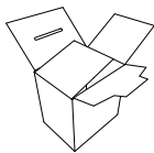
FEFCO Corrugated\0200 - Slotted Type Boxes\ FEFCO 0227 - Slotted Tuck Top and Base
