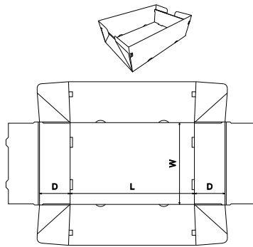
FEFCO Corrugated\0700 - Ready Glued - Self-Erecting Boxes\FEFCO 0772 - Infold Locking Tray
