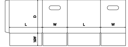
FEFCO Corrugated\0200 - Slotted Type Boxes\ FEFCO 0200 HH - Half Slotted Container Hand Holes - HSC HH
