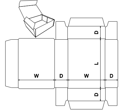
FEFCO Corrugated\0400 - Folder Type Boxes\ FEFCO 0420 - Flanged Tuck Tray
