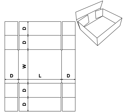
FEFCO Corrugated\0400 - Folder Type Boxes\ FEFCO 0455 - Tray Folded Sides
