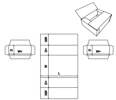
FEFCO Corrugated\0600 - Rigid Type Boxes - Bliss Boxes\FEFCO 0605 - Wrap with Part External End Caps
