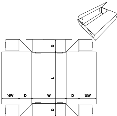
FEFCO Corrugated\0400 - Folder Type Boxes\ FEFCO 0437 - End Lock Tray, Centre Joined
