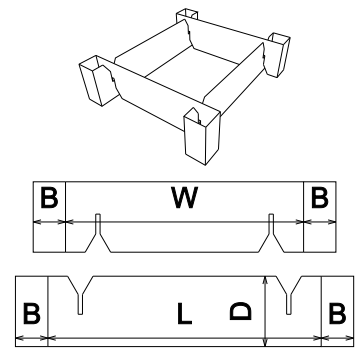
FEFCO Corrugated\0900 - Interior Fitments\ FEFCO 0932 - Interior Compartment with Reinforced Buffers
