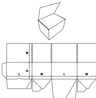
FEFCO Corrugated\0700 - Ready Glued - Self-Erecting Boxes\FEFCO 0703 - Full Crash Lock Auto Bottom, Full Overlapping Top - FCB/FOL
