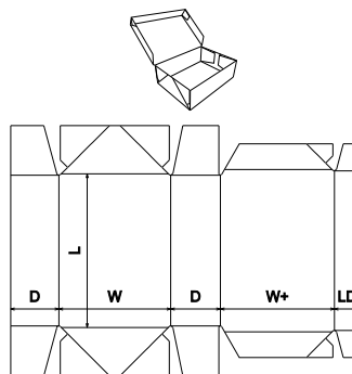
FEFCO Corrugated\0700 - Ready Glued - Self-Erecting Boxes\FEFCO 0761 - 6 Point Glued Tray with Cover
