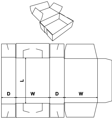
FEFCO Corrugated\0400 - Folder Type Boxes\ FEFCO 0442 - End Slit Lock Tuck Tray
