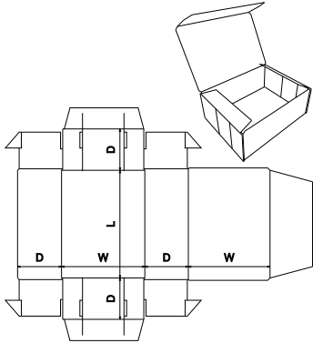
FEFCO Corrugated\0400 - Folder Type Boxes\ FEFCO 0445 - End Lock Tuck Tray
