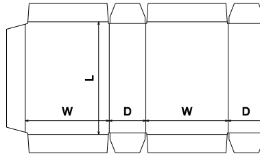
FEFCO Corrugated\0400 - Folder Type Boxes\ FEFCO 0406 - Wrap Around Blank
