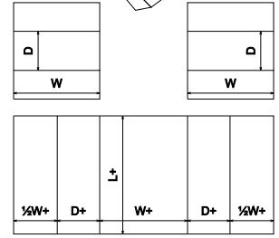
FEFCO Corrugated\0400 - Folder Type Boxes\ FEFCO 0405 - Five Panel Wrap with End Caps
