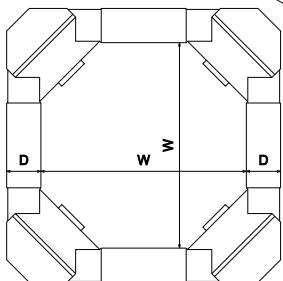
FEFCO Corrugated\0400 - Folder Type Boxes\ FEFCO 0498 - Octagonal Rolled End Tray
