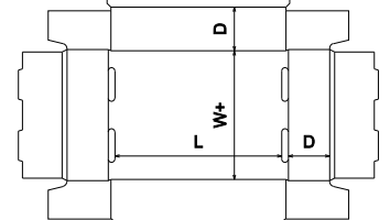
FEFCO Corrugated\0400 - Folder Type Boxes\ FEFCO 0421 - Rolled End Tuck Tray
