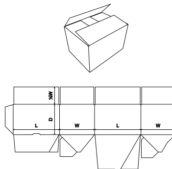
FEFCO Corrugated\0700 - Ready Glued - Self-Erecting Boxes\FEFCO 0701 - Full Crash Lock Auto Bottom, Regular Slotted Top - FCB/RSC
