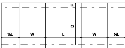
FEFCO Corrugated\0900 - Interior Fitments\ FEFCO 0913 - Fold Over Centre Seam Insert
