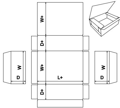
FEFCO Corrugated\0600 - Rigid Type Boxes - Bliss Boxes\FEFCO 0601 - Bliss Box with End Flaps
