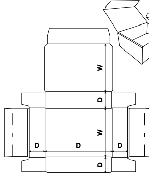
FEFCO Corrugated\0400 - Folder Type Boxes\ FEFCO 0428 - Rolled End Slot-less Tuck Tray
