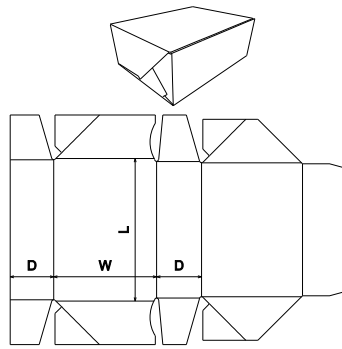
FEFCO Corrugated\0700 - Ready Glued - Self-Erecting Boxes\FEFCO 0751 - 4 Point Glued, Hinged Lid
