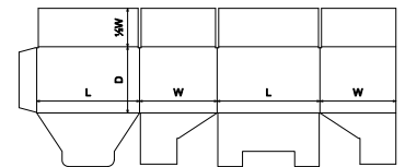
FEFCO Corrugated\0200 - Slotted Type Boxes\ FEFCO 0216 - Regular Slotted Top, Envelope Base - RSC
