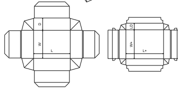
FEFCO Corrugated\0300 - Telescope Type Box\ FEFCO 0323 - Self Locking Webbed Tray and Lid
