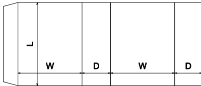
FEFCO Corrugated\0500 - Slide Type Boxes\ FEFCO 0503 - Sleeve - Top, Base and Sides
