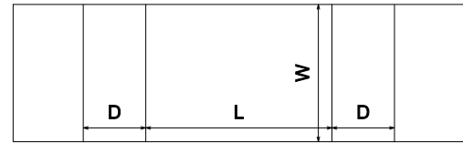
FEFCO Corrugated\0900 - Interior Fitments\ FEFCO 0907 - Tube - Over End - Centre Gap
