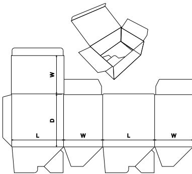
FEFCO Corrugated\0700 - Ready Glued - Self-Erecting Boxes\FEFCO 0713 - Crash Lock Base Auto Bottom, Tuck to Front Top - CLB/TF
