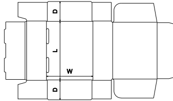
FEFCO Corrugated\0400 - Folder Type Boxes\ FEFCO 0426 - Rolled Side Tuck Tray with Dust Flaps - Pizza Box
