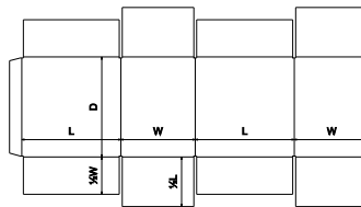
FEFCO Corrugated\0200 - Slotted Type Boxes\ FEFCO 0204 - All Flaps Meet Slotted Container - AFM - CSSC
