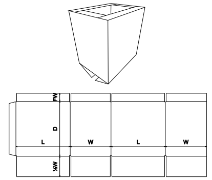
FEFCO Corrugated\0200 - Slotted Type Boxes\ FEFCO 0209 - Flange Top, Regular Slotted Base - RSC
