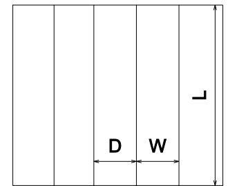
FEFCO Corrugated\0900 - Interior Fitments\ FEFCO 0914 - Tube - 5 Panel
