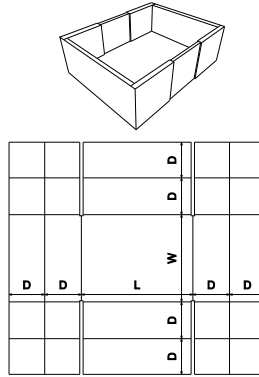
FEFCO Corrugated\0400 - Folder Type Boxes\ FEFCO 0456 - Full Reinforced Tray
