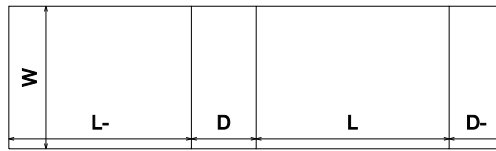
FEFCO Corrugated\0900 - Interior Fitments\ FEFCO 0905 - Tube - Over End - End Gap
