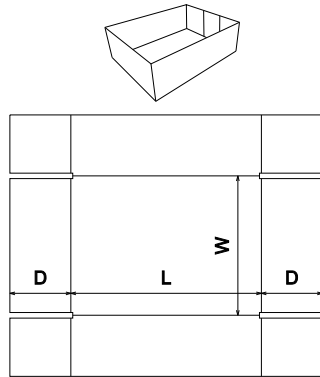
FEFCO Corrugated\0400 - Folder Type Boxes\ FEFCO 0453 - End Slotted Tray
