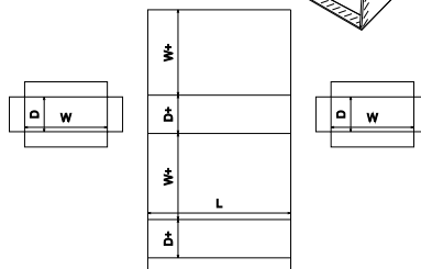
FEFCO Corrugated\0600 - Rigid Type Boxes - Bliss Boxes\FEFCO 0610 - Wrap with Internal Buffer End Caps
