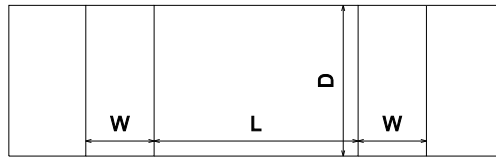
FEFCO Corrugated\0900 - Interior Fitments\ FEFCO 0908 - Tube - Side Band - Centre Gap
