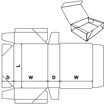
FEFCO Corrugated\0700 - Ready Glued - Self-Erecting Boxes\FEFCO 0747 - 4 Point Side Glued Tuck Tray
