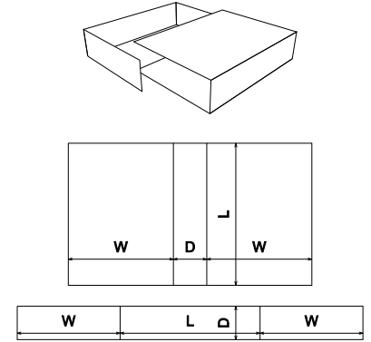
FEFCO Corrugated\0900 - Interior Fitments\ FEFCO 0929 - Interior Wraps
