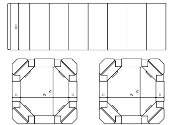
FEFCO Corrugated\0300 - Telescope Type Box\ FEFCO 0351 - Octagonal Bulk Box - Rolled Ends
