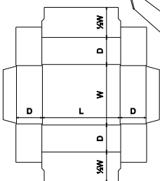
FEFCO Corrugated\0400 - Folder Type Boxes\ FEFCO 0412 - Courier Pack, Diecut Centre Taped
