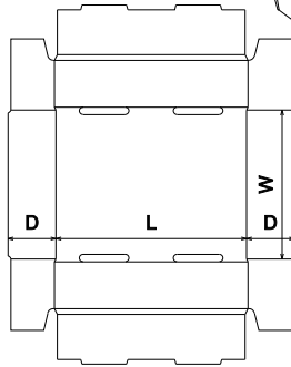
FEFCO Corrugated\0400 - Folder Type Boxes\ FEFCO 0423 - Rolled Side Tray
