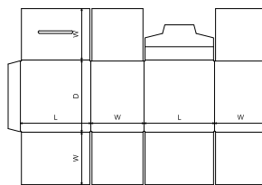
FEFCO Corrugated\0200 - Slotted Type Boxes\ FEFCO 0218 - Recloseable Top, Full Overlapping Slotted Base - FOL
