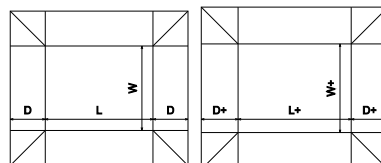
FEFCO Corrugated\0300 - Telescope Type Box\ FEFCO 0309 - Webbed Corner Tray and Lid
