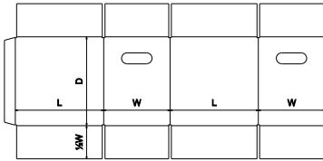
FEFCO Corrugated\0200 - Slotted Type Boxes\ FEFCO 0201 HH - Regular Slotted Container Hand Holes - RSC HH
