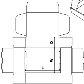
FEFCO Corrugated\0400 - Folder Type Boxes\ FEFCO 0429 - Rolled End Tuck Tray with Dust Flaps
