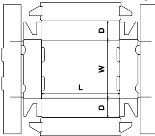
FEFCO Corrugated\0400 - Folder Type Boxes\ FEFCO 0432 - Locking Flanged Tray
