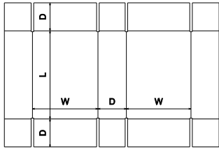
FEFCO Corrugated\0400 - Folder Type Boxes\ FEFCO 0409 - Five Panel Folder, Side Taped - FPF
