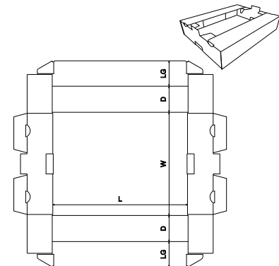
FEFCO Corrugated\0400 - Folder Type Boxes\ FEFCO 0436 - Flanged Stacking Tray
