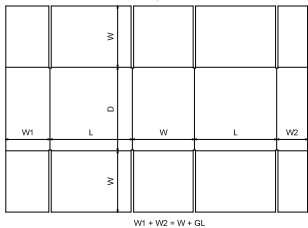
FEFCO Corrugated\0200 - Slotted Type Boxes\ FEFCO 0231 - Full Overlapping Container, Centre Seam on Ends
