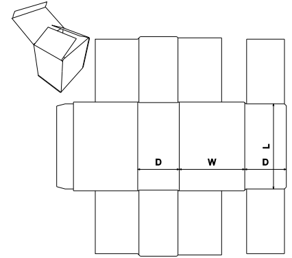
FEFCO Corrugated\0400 - Folder Type Boxes\ FEFCO 0443 - Unglued Tuck To Front
