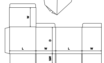
FEFCO Corrugated\0200 - Slotted Type Boxes\ FEFCO 0212 - Tuck to Front Top, Regular Slotted Base - RSC
