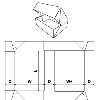
FEFCO Corrugated\0700 - Ready Glued - Self-Erecting Boxes\FEFCO 0759 - 4 Point Glued Tray with Lid
