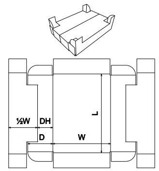
FEFCO Corrugated\0400 - Folder Type Boxes\ FEFCO 0446 - Product Tray Stand Off Corners
