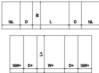
FEFCO Corrugated\0400 - Folder Type Boxes\ FEFCO 0404 - 2 Piece Folder
