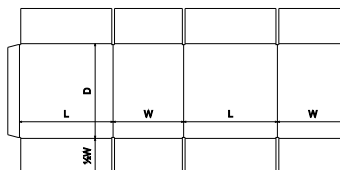
FEFCO Corrugated\0200 - Slotted Type Boxes\ FEFCO 0201 - Regular Slotted Container - RSC
