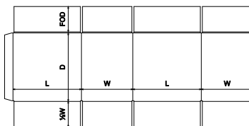
FEFCO Corrugated\0200 - Slotted Type Boxes\ FEFCO 0214 - Roll Over Top Slotted Container - RSC
