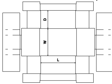
FEFCO Corrugated\0400 - Folder Type Boxes\ FEFCO 0433 - Buffered Flanged Tray
