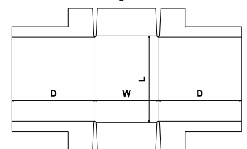
FEFCO Corrugated\0400 - Folder Type Boxes\ FEFCO 0460 - Style B - High Wall Tray - Display Tray
