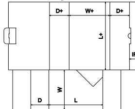
FEFCO Corrugated\0400 - Folder Type Boxes\ FEFCO 0473 - Twist Folder
