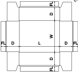
FEFCO Corrugated\0400 - Folder Type Boxes\ FEFCO 0430 - Roll Over Top Tray
