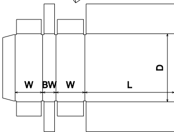
FEFCO Corrugated\0600 - Rigid Type Boxes - Bliss Boxes\FEFCO 0621 - 2 Piece Buffer Ends
