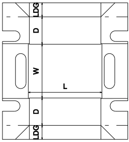
FEFCO Corrugated\0400 - Folder Type Boxes\ FEFCO 0434 - Flanged Produce Tray
