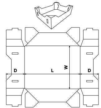
FEFCO Corrugated\0700 - Ready Glued - Self-Erecting Boxes\FEFCO 0771 - Reinforced Corner Tray
