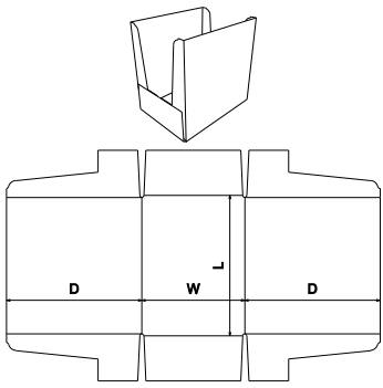
FEFCO Corrugated\0400 - Folder Type Boxes\ FEFCO 0460 - High Wall Tray - Display Tray
