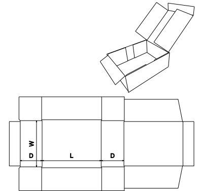
FEFCO Corrugated\0400 - Folder Type Boxes\ FEFCO 0440 - Slitted Tray Full Depth Lid
