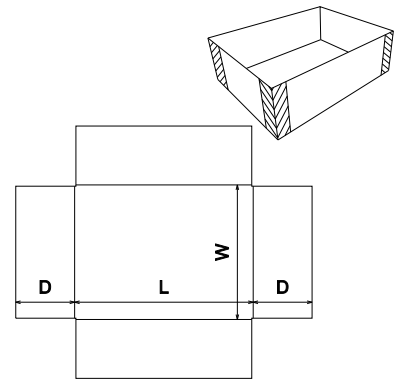
FEFCO Corrugated\0400 - Folder Type Boxes\ FEFCO 0458 - Taped Tray
