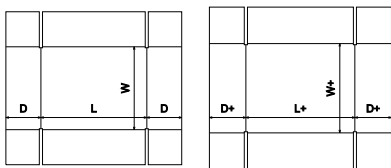
FEFCO Corrugated\0300 - Telescope Type Box\ FEFCO 0300 - Side Slotted Tray and Lid
