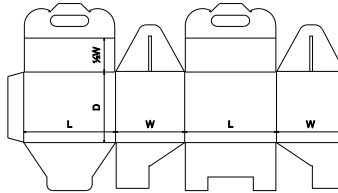
FEFCO Corrugated\0200 - Slotted Type Boxes\ FEFCO 0217 - Carry Handle Top, Envelope Base
