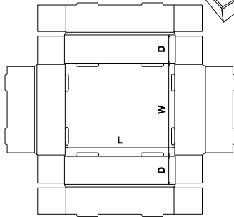
FEFCO Corrugated\0400 - Folder Type Boxes\ FEFCO 0425 - Rolled 4 Sides Tray
