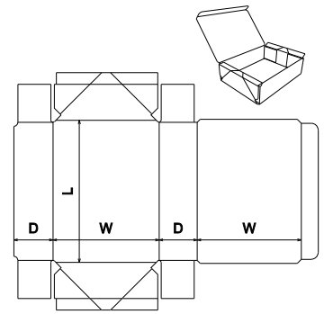
FEFCO Corrugated\0700 - Ready Glued - Self-Erecting Boxes\FEFCO 0748 - 4 Point Glued Tuck Tray
