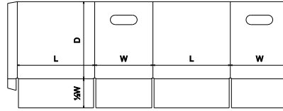
FEFCO Corrugated\0200 - Slotted Type Boxes\ FEFCO 0200 EH - Half Slotted Container Extended Gluelap Hand Holes - HSC EF HH
