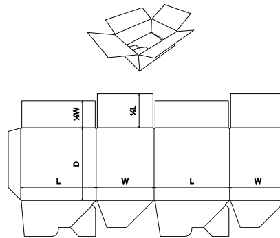
FEFCO Corrugated\0700 - Ready Glued - Self-Erecting Boxes\FEFCO 0712 - Crash Lock Base Auto Bottom, All Flaps Meet Top - CLB/AFM
