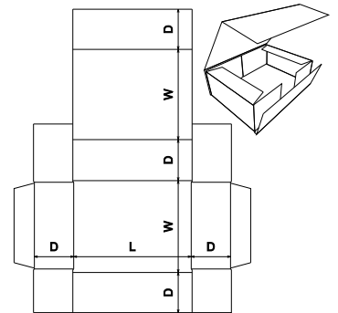
FEFCO Corrugated\0400 - Folder Type Boxes\ FEFCO 0413 - Courier Pack, Diecut Side Taped
