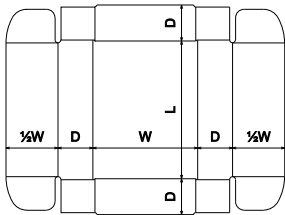
FEFCO Corrugated\0400 - Folder Type Boxes\ FEFCO 0416 - One Piece Folder, Centre Tuck - OPF
