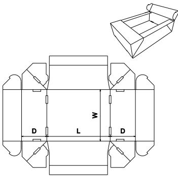
FEFCO Corrugated\0700 - Ready Glued - Self-Erecting Boxes\FEFCO 0773 - Flange Top Tray
