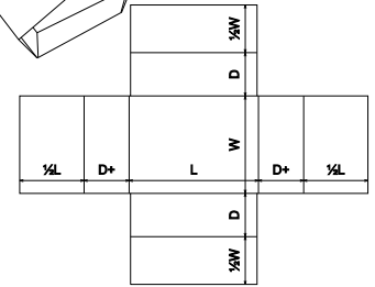
FEFCO Corrugated\0400 - Folder Type Boxes\ FEFCO 0402 - One Piece Folder, All Panels Meet - OPF
